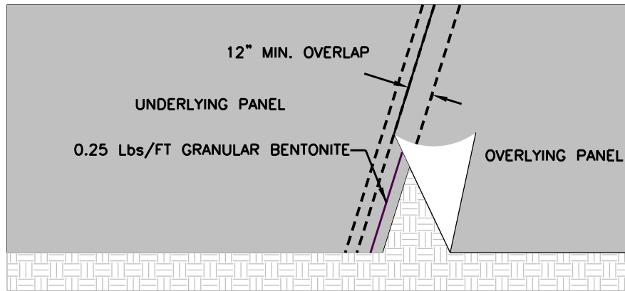
LONGITUDINAL (SIDE) SEAM DETAIL
