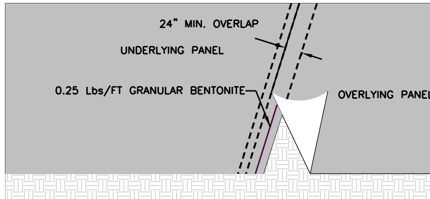
END OF PANEL (BUTT) SEAM DETAIL
